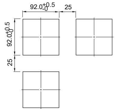
Mounting Size
