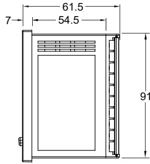
Side-face Size
